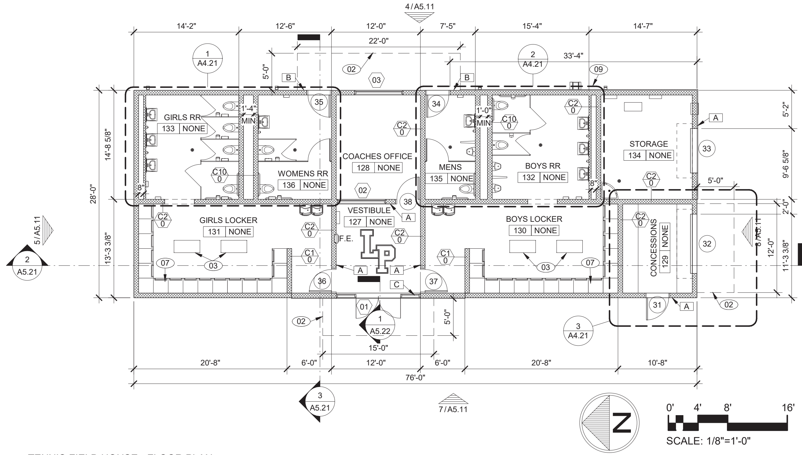
② TENNIS FIELD HOUSE - FLOOR PLAN 1/8" = 1'-0"
